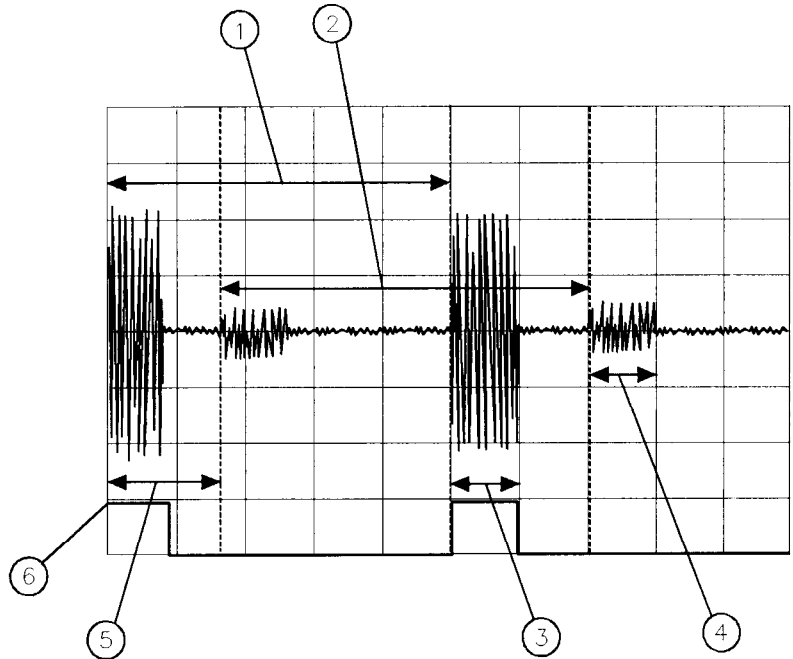
Figure 4-20. Pulse Repetition Interval and Pulse Width (with Two Signals Present)
