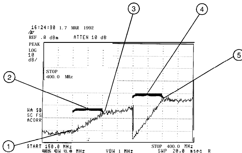
Figure 5-13. Amplitude-Correction Points
