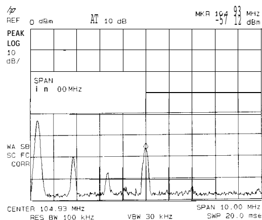
Figure 3-16. Low-Level Signal
